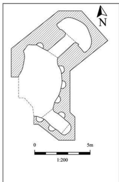
Fig. 5 Ground plan of the Grotto.
